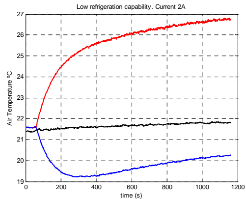
Figure 4: Result of undersized refrigeration
