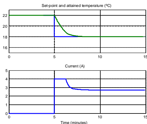
Figure 6: Dynamic response of the PI controller
