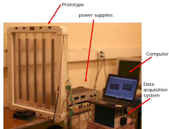
Figure 1: Experimental setup
