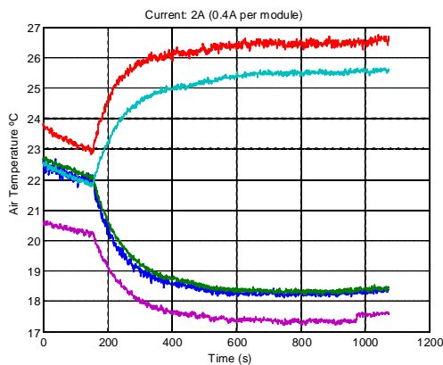
Figure 3: Temperature response. Heated air and cooled air
